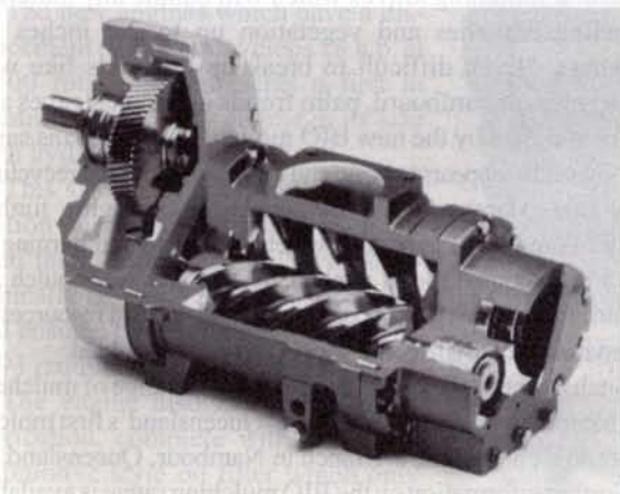
The new CompAir Cyclon series features the new air end which runs quietly and efficiently
