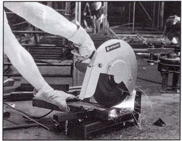
Model: G23SC – Cut-Off Machine
